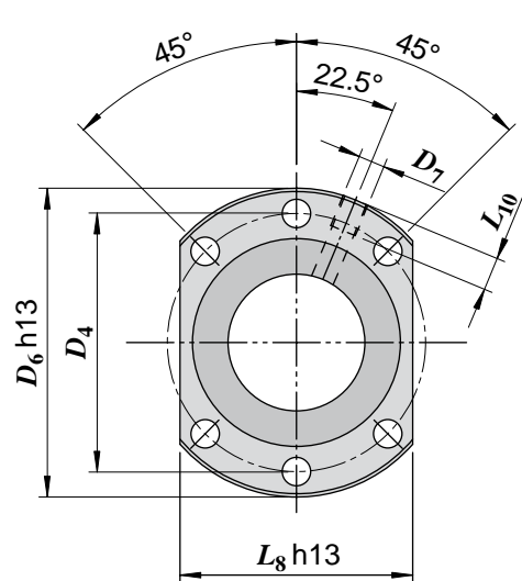
Flange type 1 ( d_0 < 40 mm)
